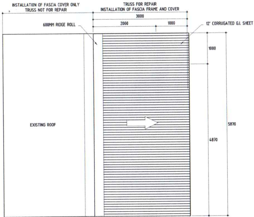
A ROOF PLAN AR-3 SCALE 1/40M
