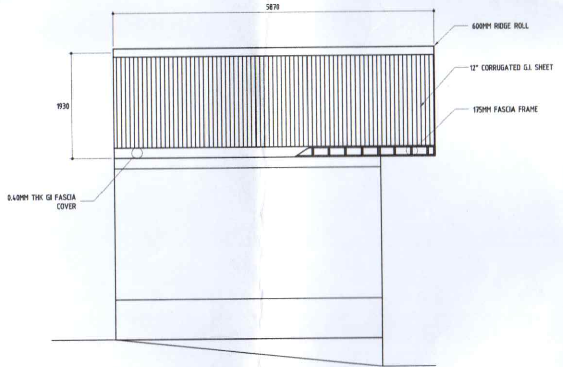
B LEFT SIDE ELEVATION AR-3 SCALE 1/40M
