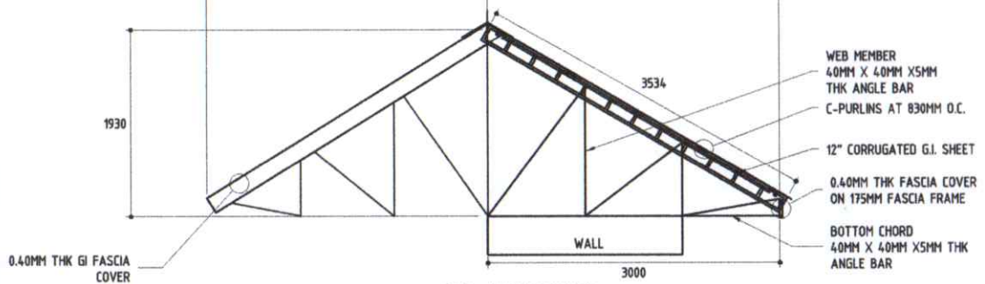
A HALF TRUSS ST-1 SCALE 1:40M
