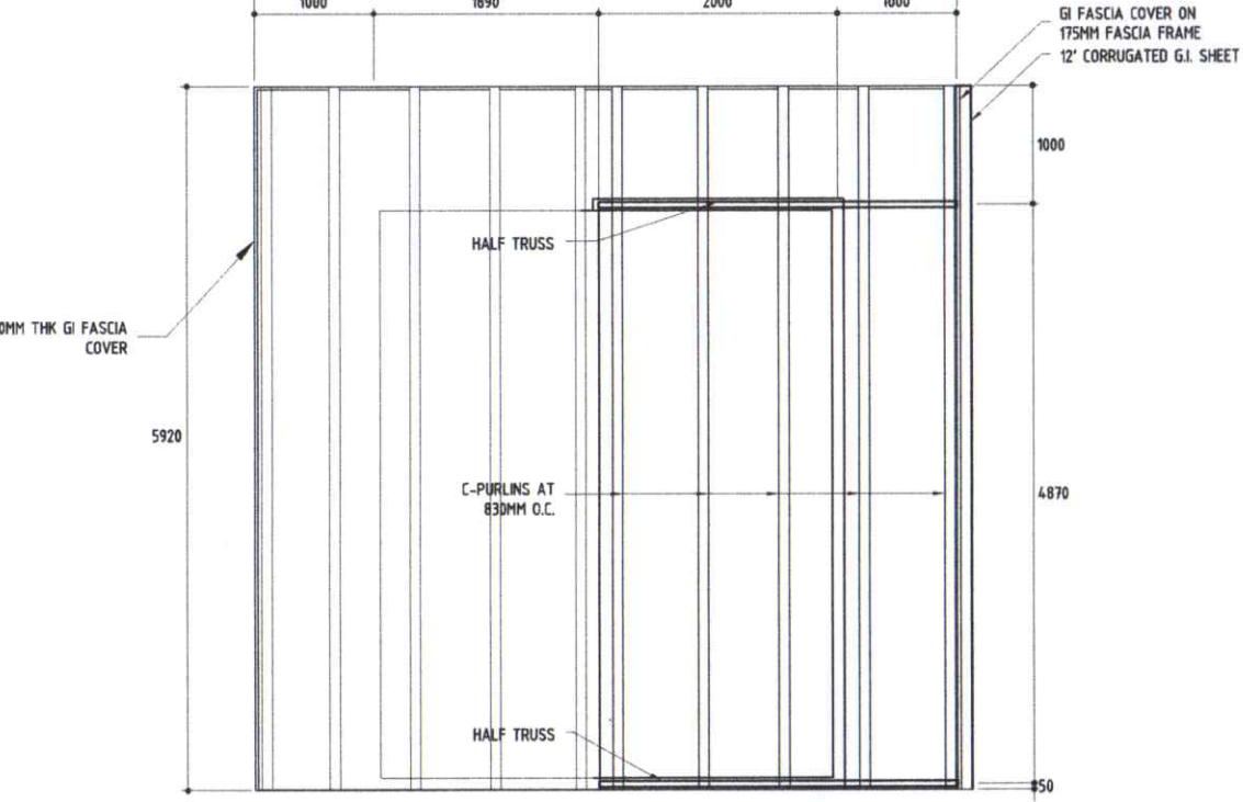
B ROOF FRAMING PLAN ST-1 SCALE 1:40M
