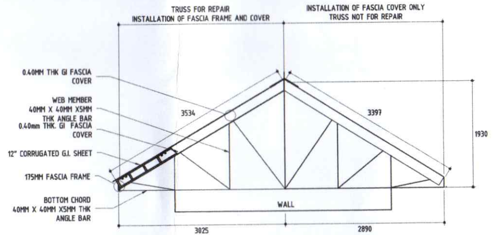
D RIGHT SIDE ELEVATION AR-3 SCALE 1/40M
