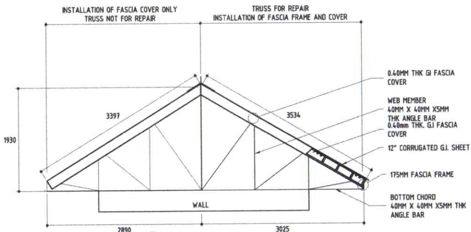
C LEFT SIDE ELEVATION AR-3 SCALE 1/40M
